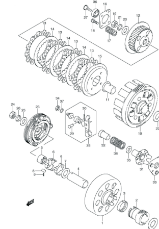
FIG.12 CLUTCH
