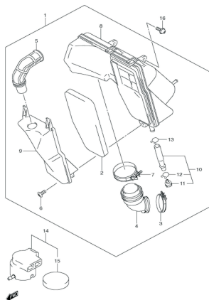
FIG.9 AIR CLEANER
