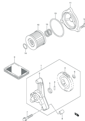
FIG.11 OIL PUMP
