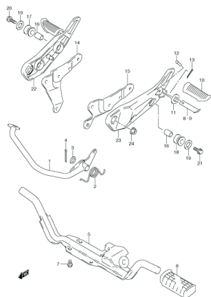
FIG.27 REAR BRAKE
