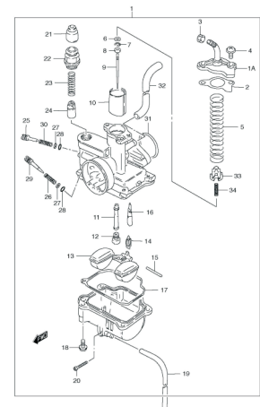
FIG.8 CARBURETOR
