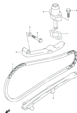
FIG.7 CAM CHAIN
