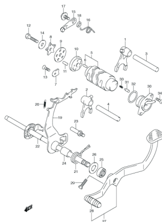
FIG.14 GEAR SHIFTING
