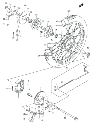
FIG.44 REAR WHEEL
