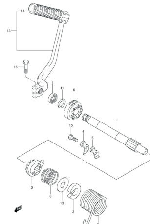
FIG.15 KICK STARTER
