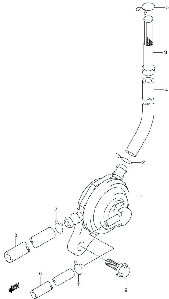
FD110CK4 P09_029 FUEL COCK
