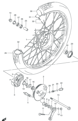
FIG.41 FRONT WHEEL
