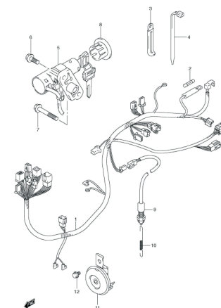
FIG.23 WIRING HARNESS
