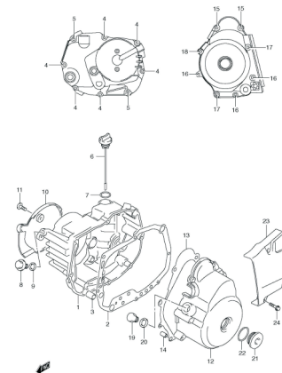
FIG.4 CRANKCASE COVERASE COVER
