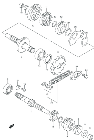
FIG.13 TRANSMISSION
