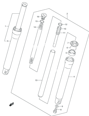
FIG.39 FRONT FORK DAMPER
