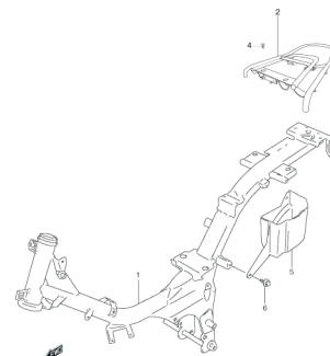
FIG.25 FRAME
