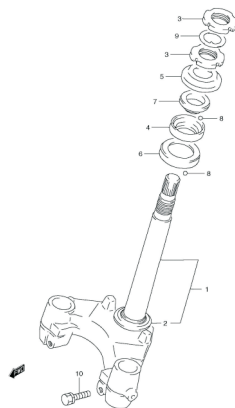
FIG.40 FRONT FORK BRACKET
