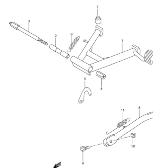
FIG.26 STAND
