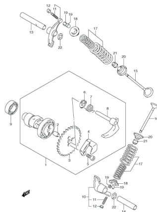
FIG.6 CAMSHAFT/VALVE
