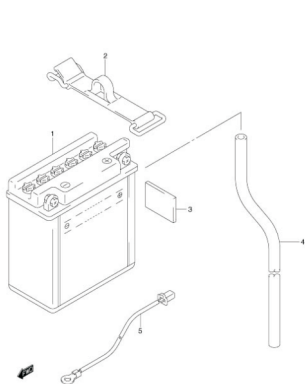
FIG.17 BATTERY
