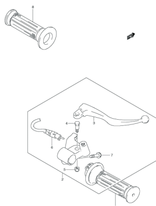
FIG.36 HANDLE LEVER
