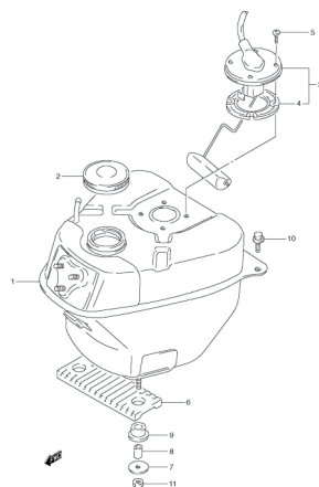
FIG.28 FUEL TANK
