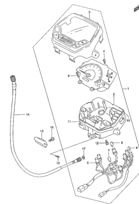
FIG.19A SPEEDOMETER
