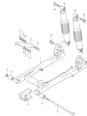
FIG.42 REAR SWINGING ARM
