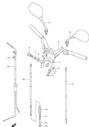
FIG.35 HANDLEBAR
