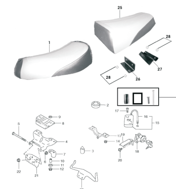
FIG.38 SEAT
