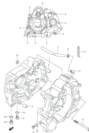
FIG.3 CRANKCASE
