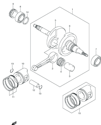
FIG.5 CRANKSHAFT
