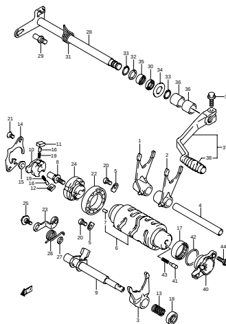
FIG.22 GEAR SHIFTING (E-5)
