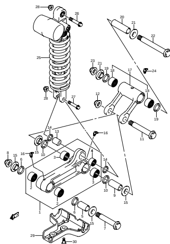
FIG.52 REAR CUSHION LEVER (I-8)
