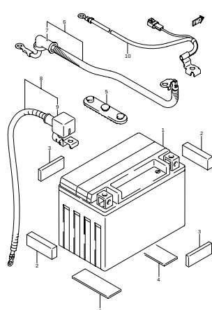
FIG.26 BATTERY (E-10)
