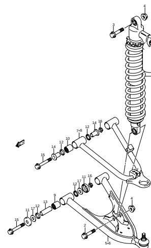
FIG.46 SUSPENSION ARM (I-2)
