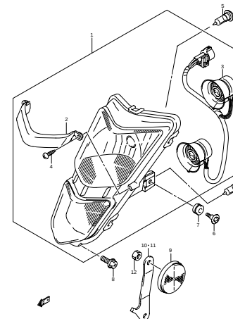
FIG.27A HEADLAMP (LT-Z400Z) (F-3)
