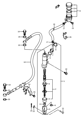
FIG.56 REAR MASTER CYLINDER (J-5)
