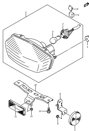
FIG.29 REAR COMBINATION (E28) (F-5)
