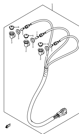
FIG.30 PILOT LAMP (F-6)
