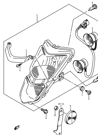
FIG.27 HEADLAMP (LT-Z400) (F-2)
