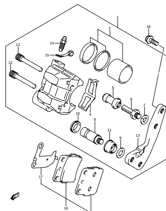
FIG.48 FRONT CALIPER (I-4)
