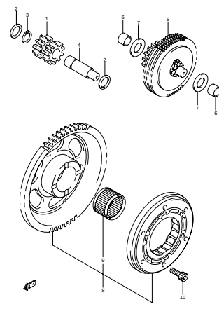
FIG.8 STARTER CLUTCH (C-2)
