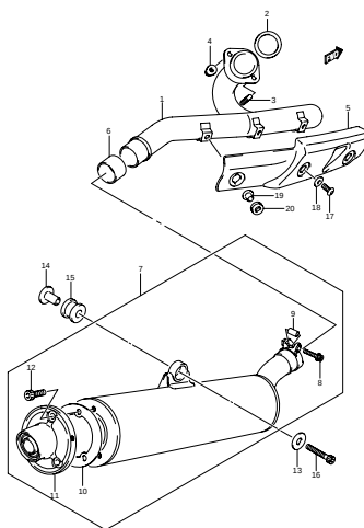
FIG.14 MUFFLER (C-10)
