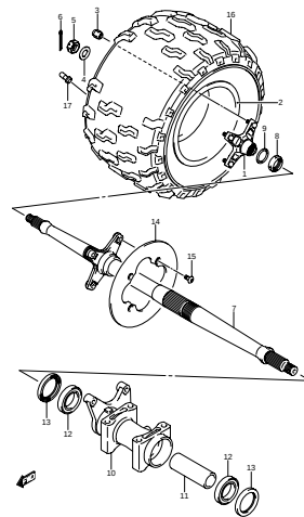
FIG.53 RIGHT REAR WHEEL (J-2)
