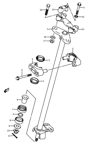
FIG.45 STEERING SHAFT (H-8)
