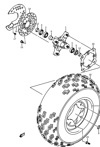
FIG.47 FRONT WHEEL (I-3)
