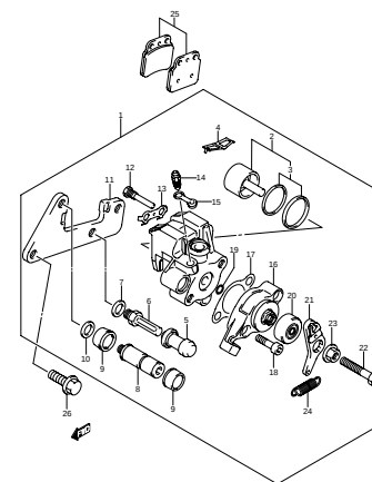
FIG.55 REAR CALIPER (J-4)
