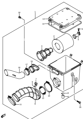
FIG.13 AIR CLEANER (C-9)
