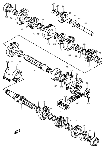
FIG.21 TRANSMISSION (E-3)
