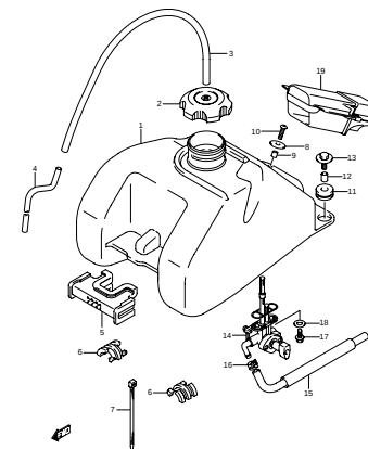
FIG.35 FUEL TANK (G-5)
