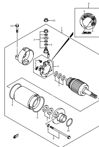
FIG.23 STARTING MOTOR (E-7)
