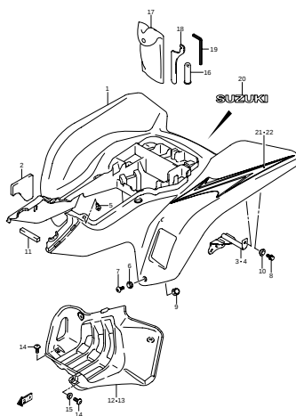
FIG.41 REAR FENDER (H-4)
