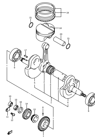
FIG.7 CRANKSHAFT (B-8)
