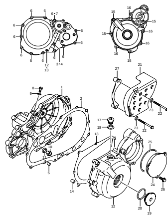
FIG.6 CRANKCASE COVER (B-7)
