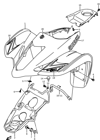
FIG.36 FRONT FENDER (G-6)
