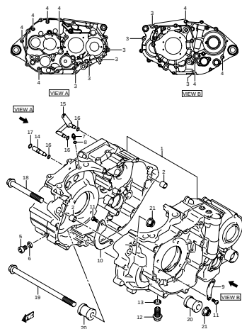
FIG.5 CRANKCASE (B-6)
