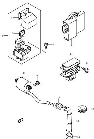
FIG.25 ELECTRICAL (E-9)
