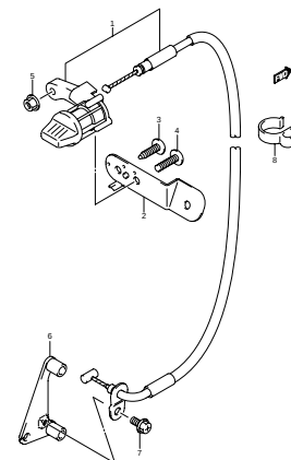
FIG.39 REVERSE LOCK (G-9)
