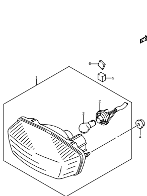
FIG.28 REAR COMBINATION (E33) (F-4)
