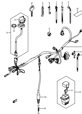
FIG.31 WIRING HARNESS (F-7)
