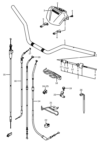
FIG.38 HANDLEBAR (G-8)
