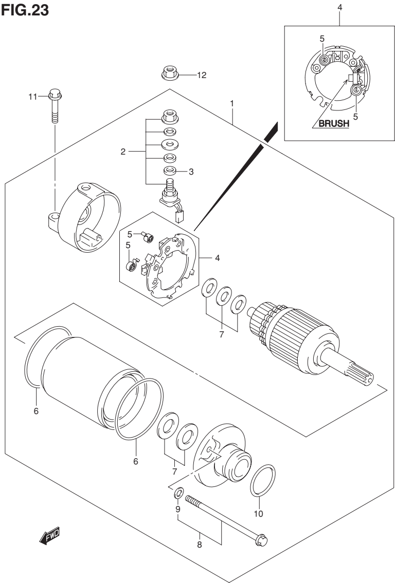
FIG.23 (E-7) STARTING MOTOR
