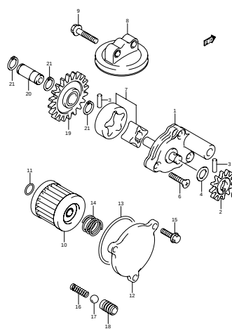
FIG.15 OIL PUMP (D-2)
