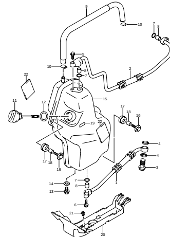
FIG.16 OIL HOSE (D-3)
