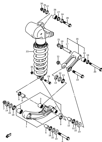
FIG.53A REAR CUSHION LEVER (MODEL K8) (H-10)
