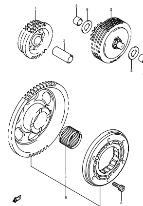
FIG.8 STARTER CLUTCH (B-9)
