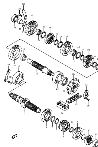
FIG.22 TRANSMISSION (MODEL K6/K7) (D-4)
