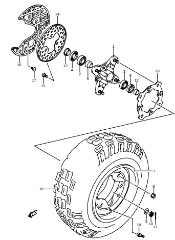
FIG.48 FRONT WHEEL (H-2)
