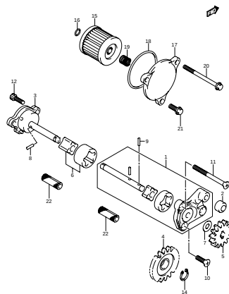
FIG.15 OIL PUMP (C-3)
