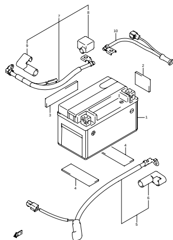
FIG.27 BATTERY (E-5)
