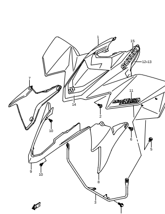
FIG.39A FRONT FENDER (MODEL K7) (F-11)
