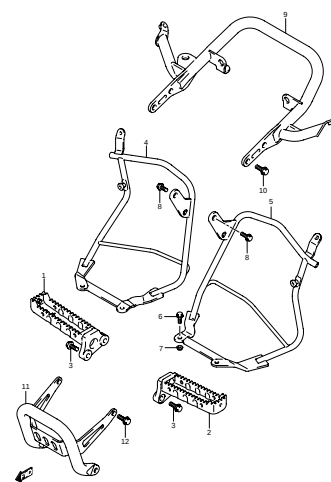
FIG.36 FOOTREST (F-5)
