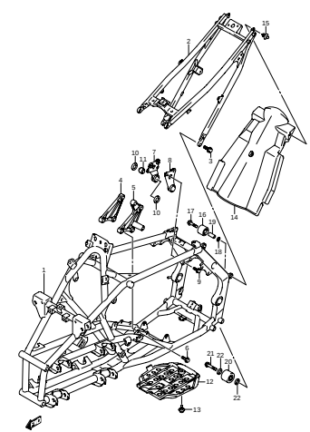
FIG.33 FRAME (F-2)
