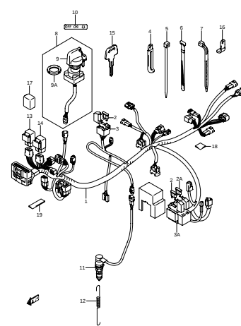
FIG.32 WIRING HARNESS (E-10)
