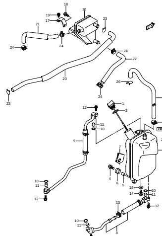
FIG.16 OIL HOSE (C-4)
