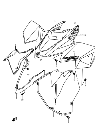
FIG.39 FRONT FENDER (MODEL 6) (F-10)
