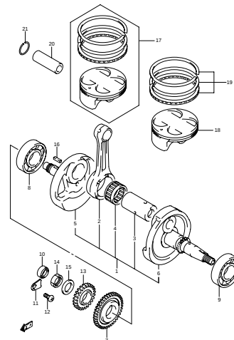
FIG.7 CRANKSHAFT (B-8)
