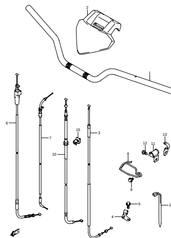
FIG.40 HANDLEBAR (F-14)
