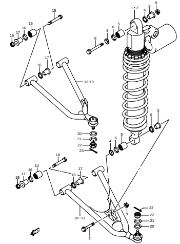
FIG.47 SUSPENSION ARM (G-10)
