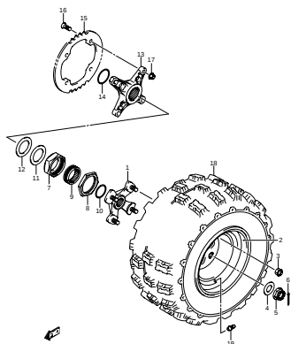
FIG.55 LEFT REAR WHEEL (MODELK 6/K7) (I-2)
