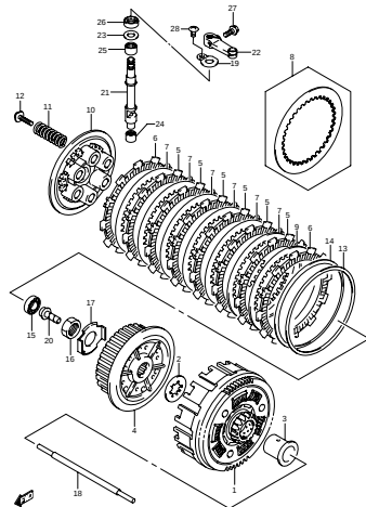
FIG.21 CLUTCH (MODEL K6/K7) (D-2)
