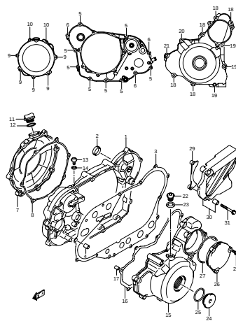
FIG.6 CRANKCASE COVER (B-7)
