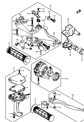
FIG.41 HANDLE LEVER (G-2)
