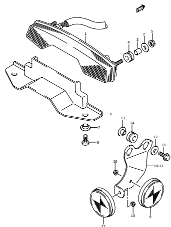
FIG.30 REAR COMBINATION (LT-R450K6/K7/ K8/ZK8 E28) (E-8)
