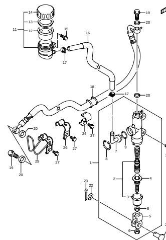
FIG.57 REAR MASTER CYLINDER (I-5)
