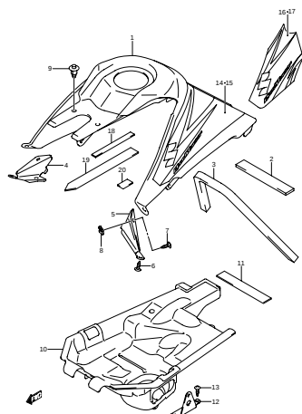
FIG.38 FUEL TANK COVER (MODEL K6/K7) (F-8)
