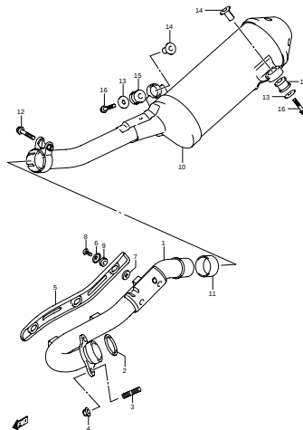
FIG.14 MUFFLER (C-2)
