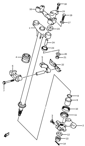
FIG.46 STEERING SHAFT (G-9)
