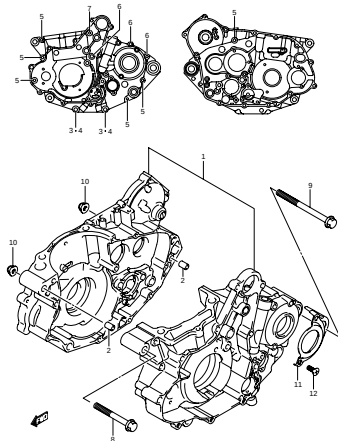
FIG.5 CRANKCASE (B-6)
