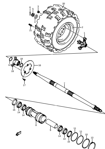
FIG.54A RIGHT REAR WHEEL (MODEL K8) (H-13)
