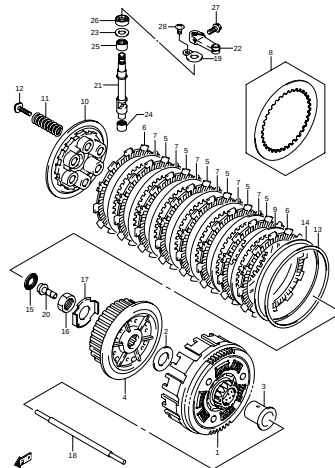
FIG.21A CLUTCH (MODEL K8) (D-3)
