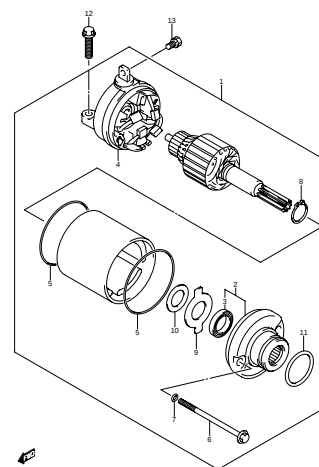
FIG.24 STARTING MOTOR (E-2)
