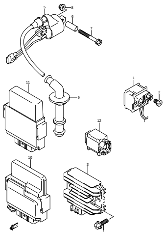
FIG.26 ELECTRICAL (E-4)
