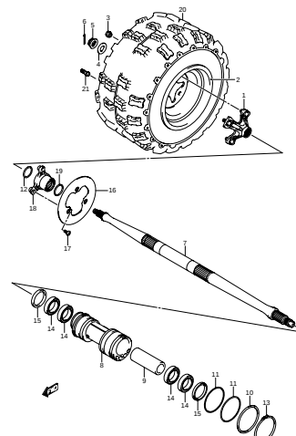
FIG.54 RIGHT REAR WHEEL (MODEL K6/K7) (H-12)
