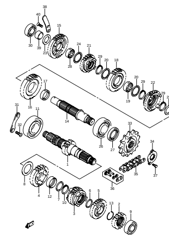
FIG.22A TRANSMISSION (MODEL K8) (D-6)
