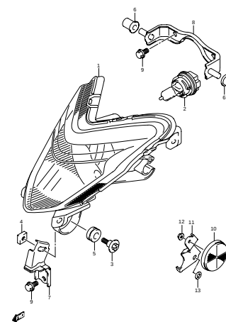
FIG.28 HEADLAMP (E-6)
