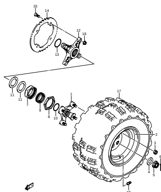
FIG.55A LEFT REAR WHEEL (MODELK 8) (I-3)
