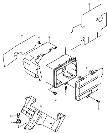
FIG.34 BATTERY HOLDER (F-3)
