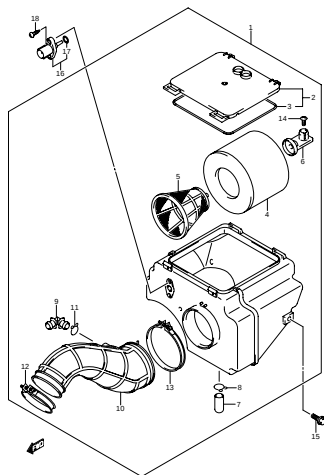
FIG.13 AIR CLEANER (B-15)
