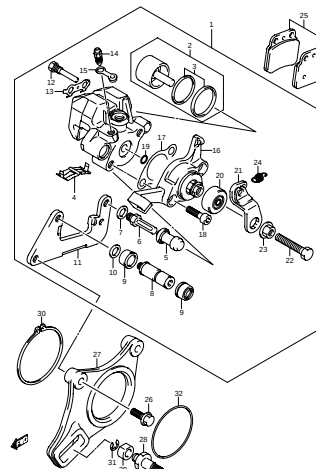
FIG.56 REAR CALIPER (I-4)
