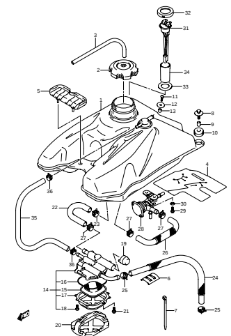
FIG.37 FUEL TANK (F-6)
