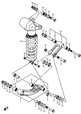
FIG.53 REAR CUSHION LEVER (MODEL K6/K7) (H-8)
