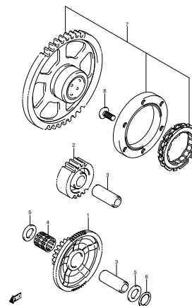
FIG.8 STARTER CLUTCH (B-10)
