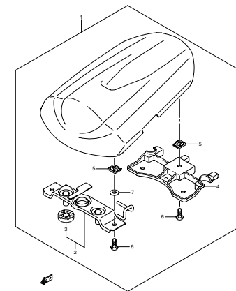
FIG.56 SEAT TAIL BOX (H-3)
