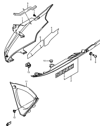
FIG.53 UNDER COWLING (G-14)
