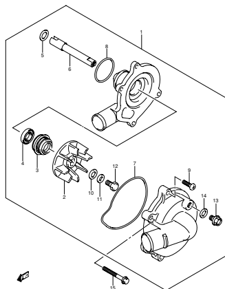
FIG.18 WATER PUMP (C-8)
