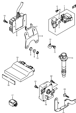
FIG.29 ELECTRICAL (D-12)
