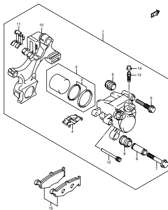
FIG.66 REAR CALIPER (H-13)
