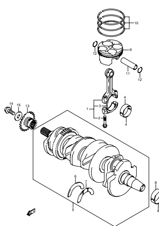
FIG.7 CRANKSHAFT (B-9)
