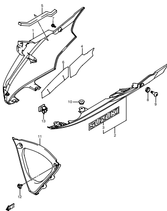
FIG.53A UNDER COWLING (MODEL K9) (G-15)
