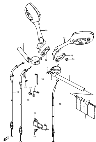
GSX-R750K8 E03 E28_045 HANDLE BAR
