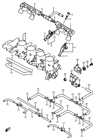
FIG.13 THROTTLE BODY HOSE/JOINT (C-3)
