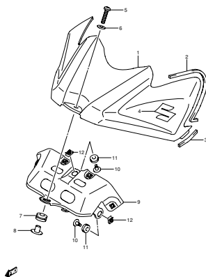
FIG.42A FRAME COVER (MODEL K9) (F-12)
