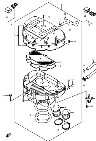
FIG.14 AIR CLEANER (C-4)
