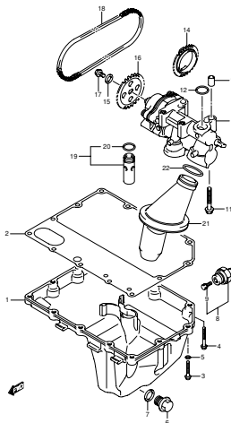
FIG.6 OIL PAN · OIL PUMP (B-8)
