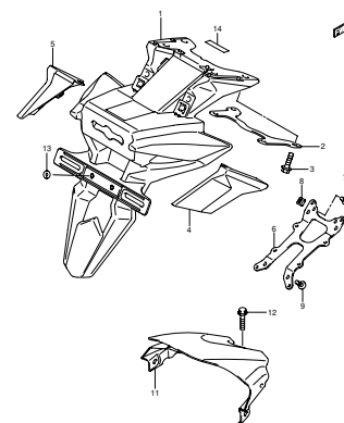
GSX-R750K8 E03 E28_048 REAR FENDER LOWER
