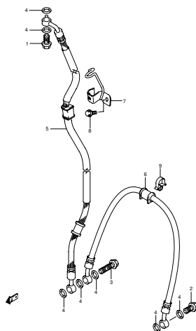
FIG.61 FRONT BRAKE HOSE (H-8)
