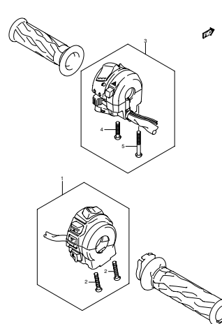
FIG.35 HANDLE SWITCH (E-6)
