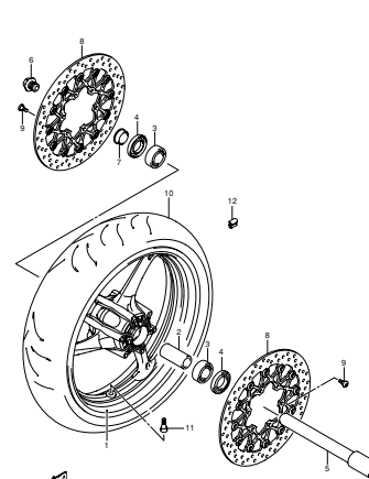
FIG.59 FRONT WHEEL (H-6)
