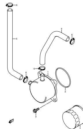
FIG.16 OIL COOLER (C-6)
