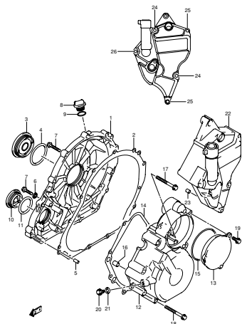
FIG.5 CRANKCASE COVER (B-7)
