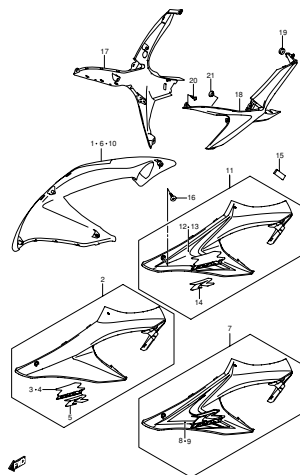
FIG.54 LABEL (G-16)
