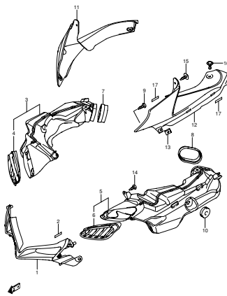
GSX-R750KB E03 E28_050 AIR INTAKE PIPE
