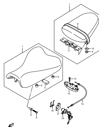
FIG.55 SEAT (H-2)
