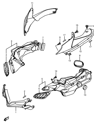
GSX-R750K8 E03 E28_050A AIR INTAKE PIPE
