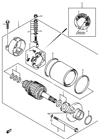
FIG.29 ELECTRICAL (D-12)
