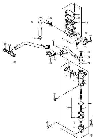
FIG.67 REAR MASTER CYLINDER (H-14)
