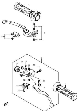
GSX-R750K8 E03 E28_046 HANDLE LEVER
