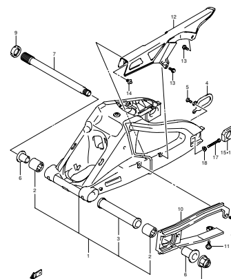
FIG.63 REAR SWINGING ARM (H-10)
