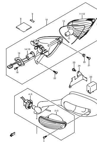
FIG.32 TURN SIGNAL LAMP (E-2)
