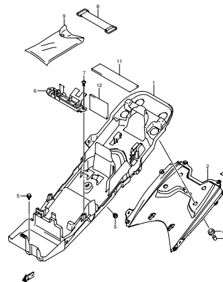
GSX-R750K8 E03 E28_047 REAR FENDER UPPER
