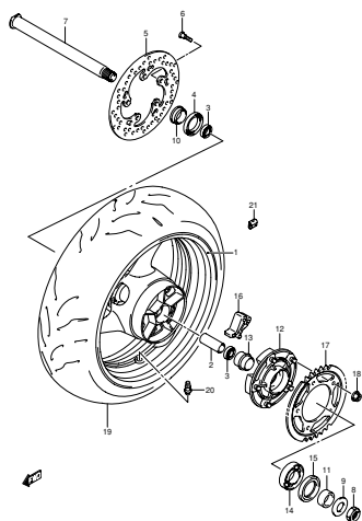
FIG.65 REAR WHEEL (H-12)
