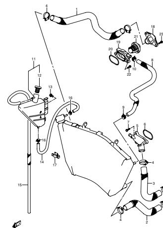
FIG.20 RADIATOR HOSE (C-10)
