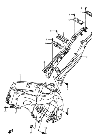
FIG.36 FRAME (F-2)
