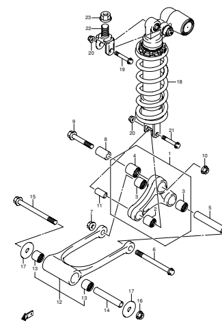
FIG.64 REAR CUSHION LEVER (H-11)
