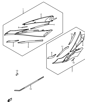
FIG.43A FRAME SIDE COVER (MODEL K9) (F-15)
