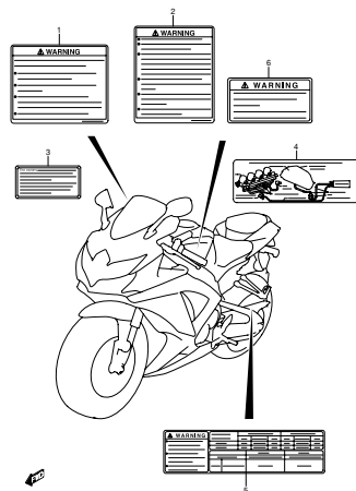
FIG.54 LABEL (G-16)
