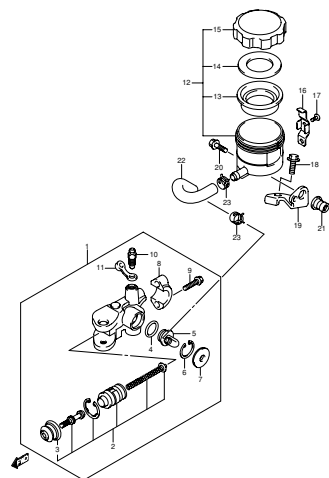
FIG.62 FRONT MASTER CYLINDER (H-9)
