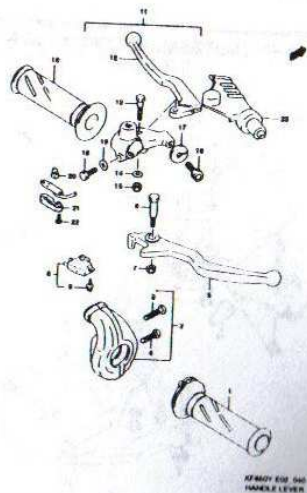
FIG. 40 HANDLE LEVER (F-11)
