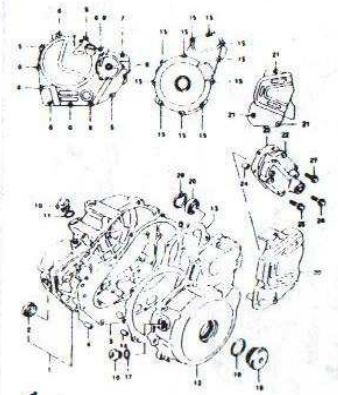
FIG. 4 CRANKCASE COVER (B-5)
