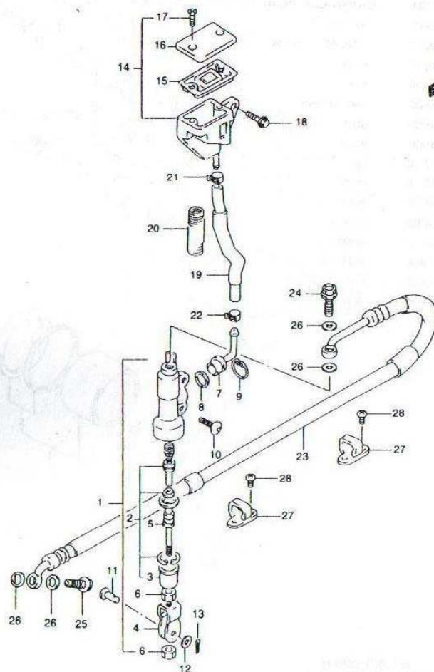
XF650Y E02_056 REAR MASTER CYLINDER
