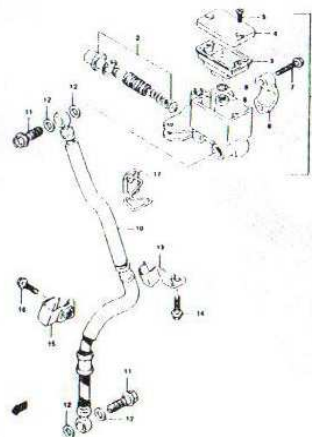
FIG. 51 FRONT MASTER CYLINDER (MODEL V/W/X) (H-6)
