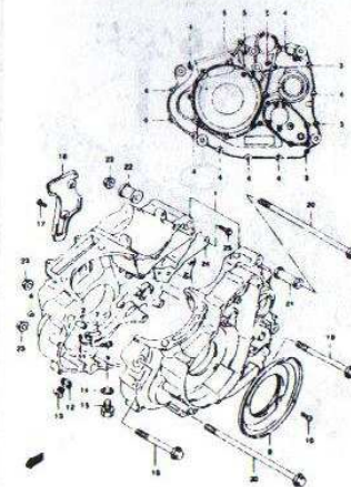
FIG. 3 CRANKCASE (B-4)
