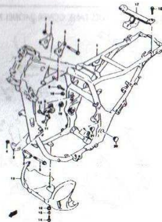
FIG. 30 FRAME (E-2)
