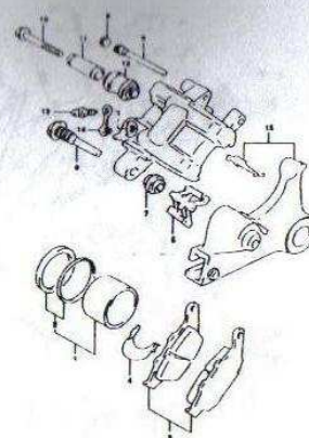
FIG. 55A REAR CALIPER (MODEL X/Y) (H-12)
