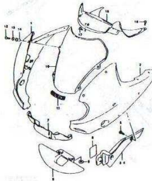
FIG. 42B COWLING (MODEL X) (G-4)
