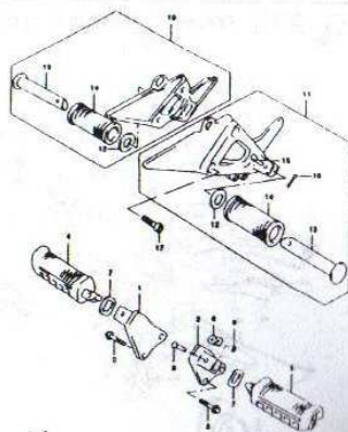
FIG. 33 FOOTREST (E-5)
