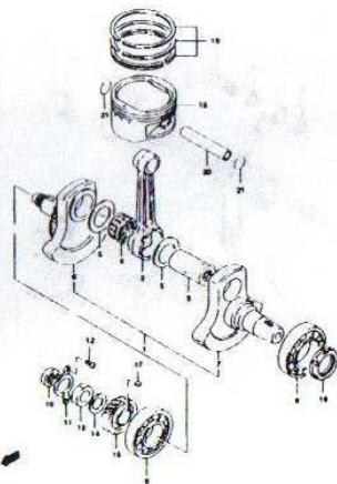
FIG. 5 CRANKSHAFT (B-6)
