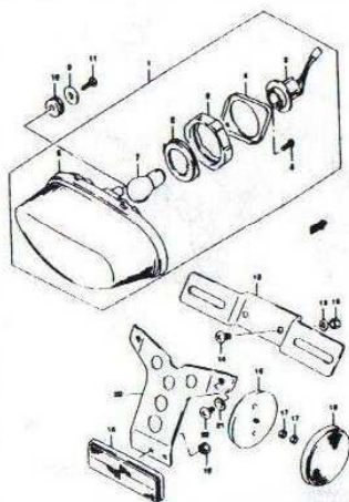
FIG. 27 REAR COMBINATION LAMP (D-12)
