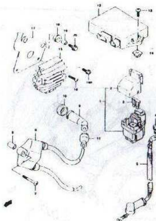
FIG. 23 ELECTRICAL (D-5)
