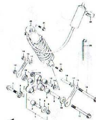
FIG. 53 REAR CUSHION LEVER (H-9)
