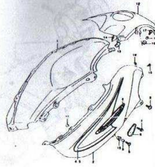
FIG. 35C FUEL TANK COVER (MODEL Y) (E-10)
