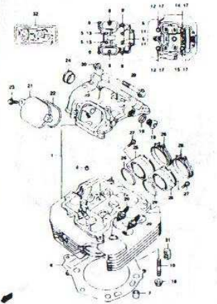
FIG. 1 CYLINDER HEAD (B-2)
