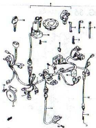
FIG. 28A WIRING HARNESS (MODEL Y) (D-14)
