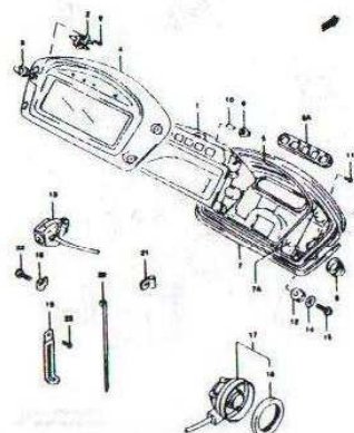
FIG. 24 SPEEDOMETER (D-6)
