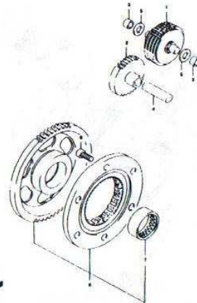
FIG. 6 STARTER CLUTCH (B-7)
