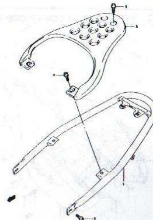
FIG. 31 CARRIER (E-3)
