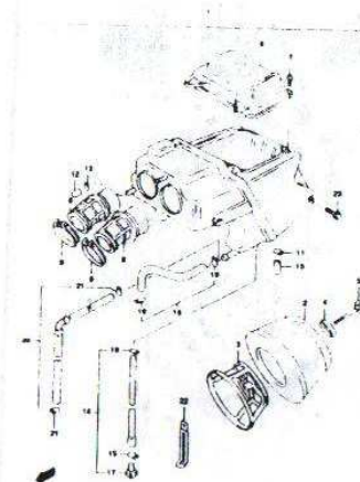
FIG. 11 AIR CLEANER (C-5)
