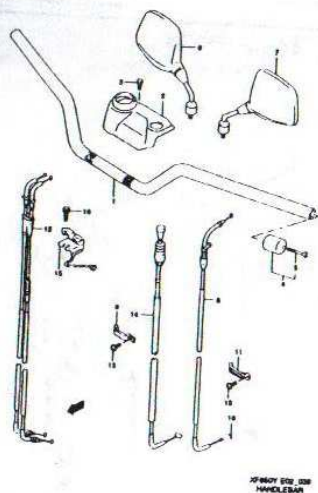
FIG. 39 HANDLEBAR (F-10)
