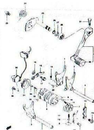
FIG. 19 GEAR SHIFTING (C-14)
