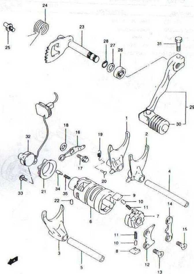
XF650Y E02_019 GEAR SHIFTING
