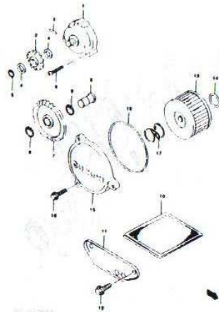
FIG. 13 OIL PUMP (C-7)
