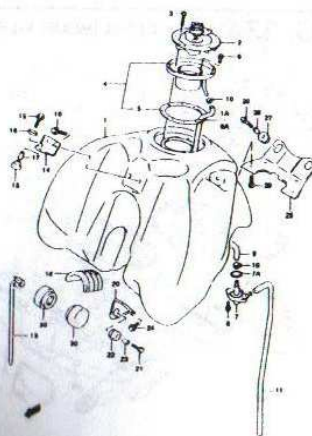
FIG. 34 FUEL TANK (E-6)
