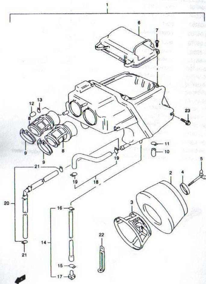
XF650F E02_011 AIR CLEANER
