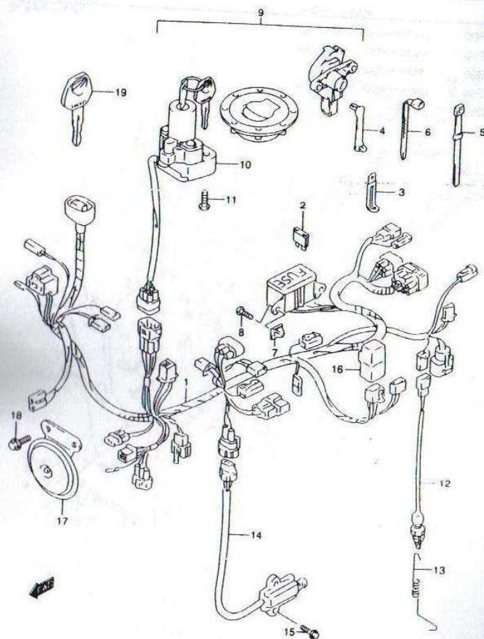
XF650Y E02_028A WIRING HARNESS(Y)
