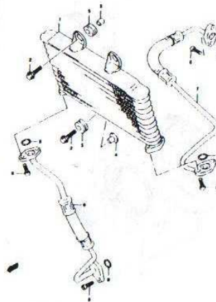
FIG. 14 OIL COOLER (C-8)
