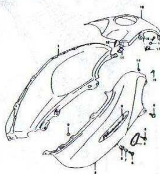
FIG. 35B FUEL TANK COVER (MODEL X) (E-9)
