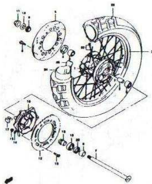
FIG. 54 REAR WHEEL (H-10)
