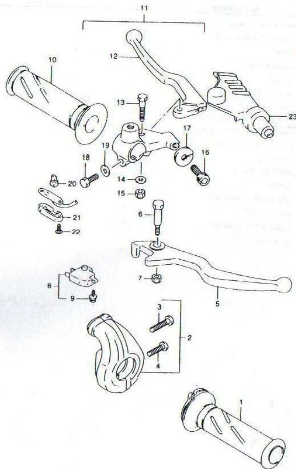
XF650Y E02_040 HANDLE LEVER
