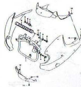
FIG. 43 COWLING INSTALLATION PARTS (MODEL V/W/X) (G-6)
