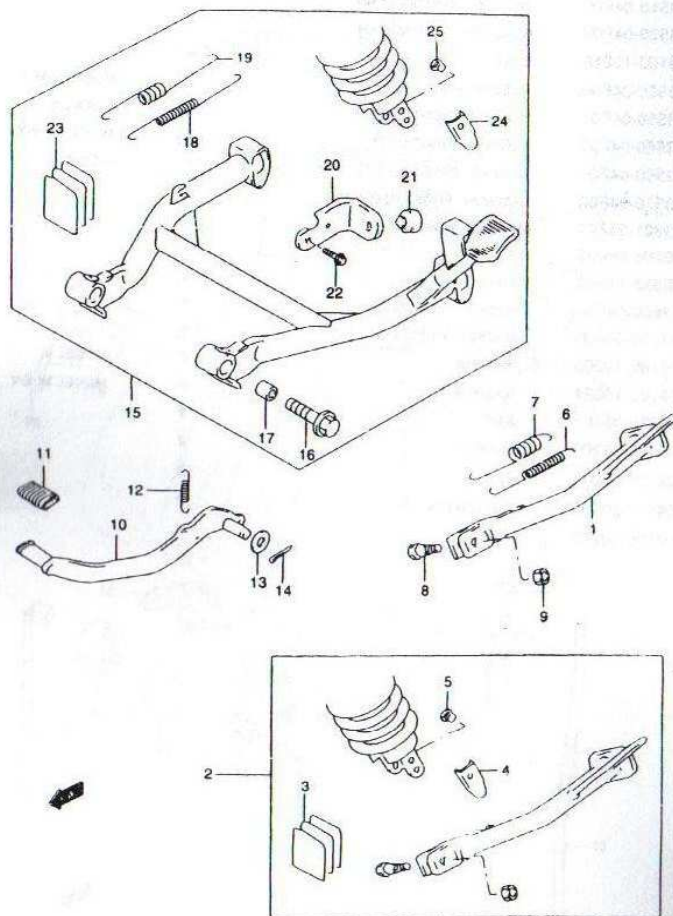
XF650Y E02_032 STAND
