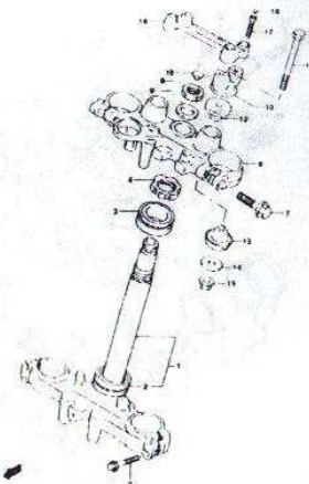
FIG. 48 STEERING STEM (H-3)
