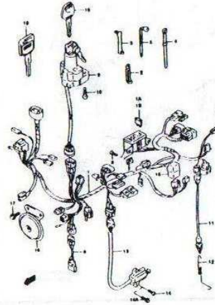
FIG. 28 WIRING HARNESS (MODEL V/W/X) (D-13)
