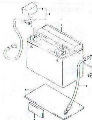
FIG. 22 BATTERY (D-4)
