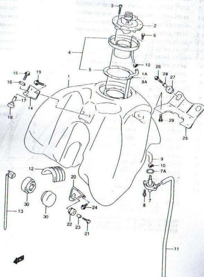
XF650Y E02_034 FUEL TANK
