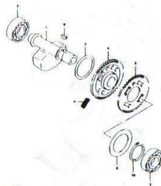
FIG. 7 CRANK BALANCER (B-8)
