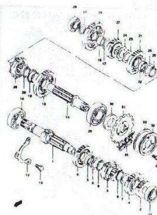
FIG. 18 TRANSMISSION (C-12)
