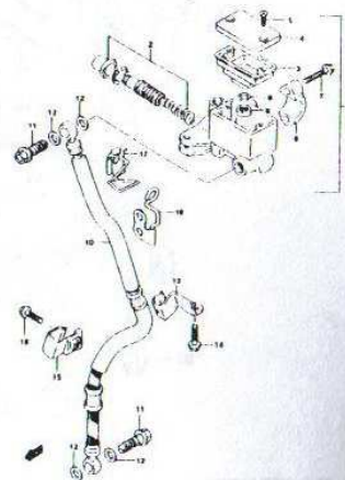
FIG. 51A FRONT MASTER CYLINDER (MODEL Y) (H-7)
