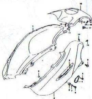
FIG. 35A FUEL TANK COVER (MODEL W) (E-8)
