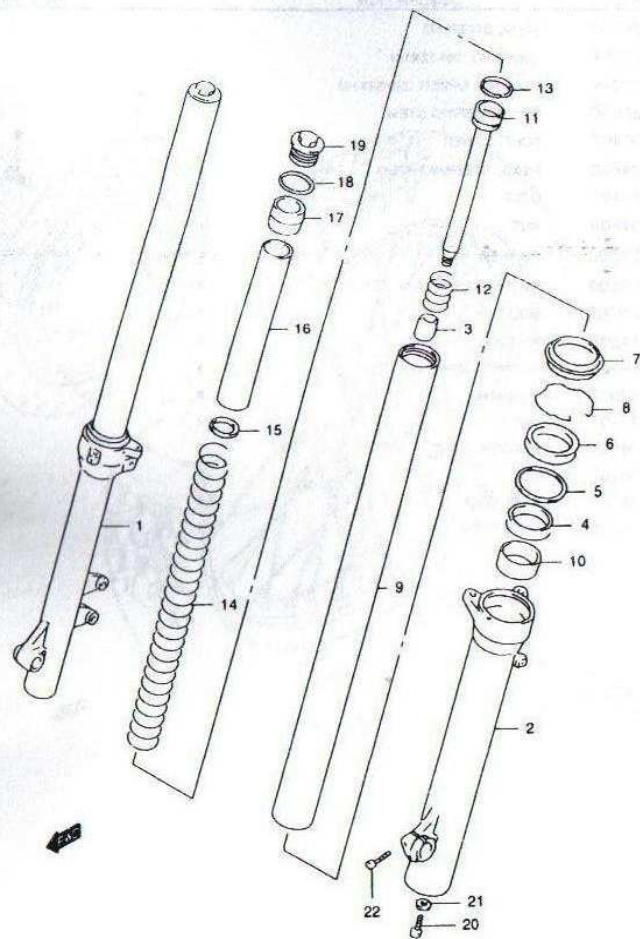
XF650Y E02_047 FRONT DAMPER
