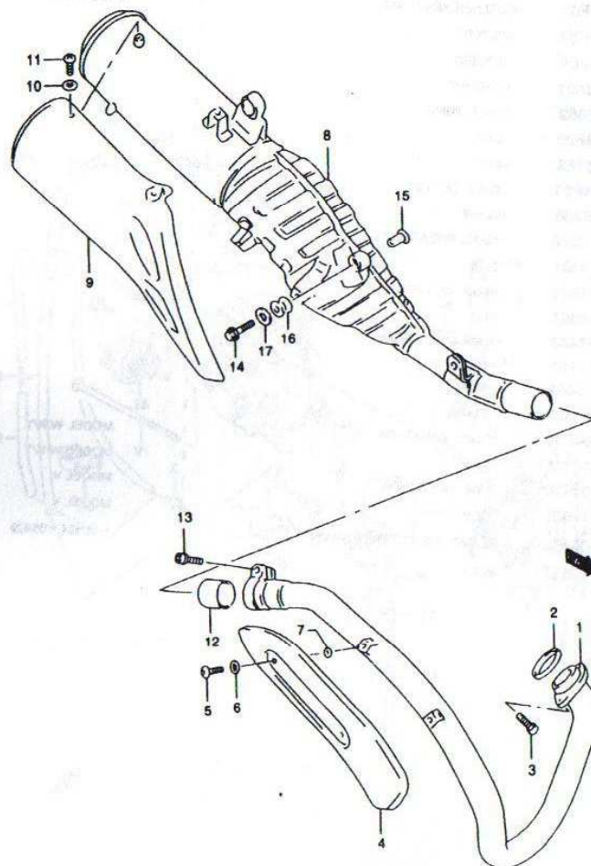
XF650Y E02_012 MUFFLER
