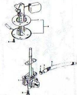
FIG. 36 FUEL COCK (E-11)
