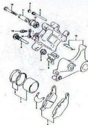
FIG. 55 REAR CALIPER (MODEL V/W) (H-11)
