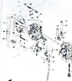
FIG. 10A CARBURETOR FITTINGS (C-4)
