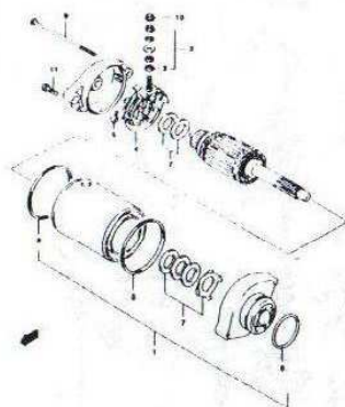
FIG. 20 STARTING MOTOR (D-2)
