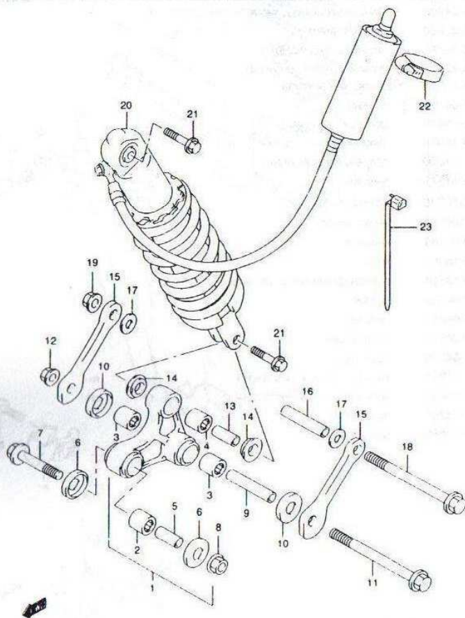
XF650Y E02_053 REAR CUSHION LEVER
